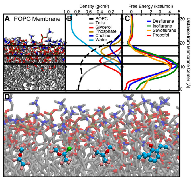
Fig. 4. Partitioning profiles of inhaled anesthetics into a POPC membrane. A) Snapshot of the POPC membrane used in the simulations. Water and ions are omitted for clarity. The color of the atom groups in this image corresponds to the color of the curves in the density profiles. B) Density profile of the simulated systems used to demarcate the regions of the membrane for analysis of anesthetic–membrane interactions. Here, total POPC density is shown as the black dashed line and water density is shown as the light blue line. POPC density was further subdivided into tail (gray), glycerol (red), phosphate (gold), and choline (blue) density. The colors of the curves correspond to the color of the atoms shown in (a). C) PMF for inserting desflurane (blue), isoflurane (green), sevoflurane (orange), and propofol (red) into the membrane. All anesthetics show a distinct energy minimum at the interfacial region, while there is negligible energy difference between the bulk aqueous environment and midpoint of the lipid bilayer. D) Representative snapshot of (starting on left and moving right) desflurane, isoflurane, sevoflurane, and propofol in the umbrella sampling simulations showing the low energy conformation at the amphipathic boundary of the membrane. Figure reprinted from Arcario et al. [89].
