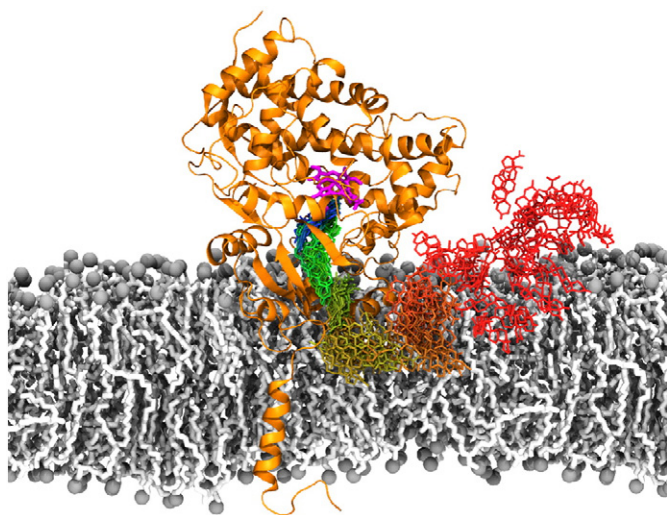
Fig. 7. Membrane-mediated drug binding mechanism of CYP3A4. The binding pathway of progesterone was reconstructed by combining independent equilibrium simulations of progesterone along the putative access tunnel (shown in green-to-blue colorscale, stick representation), and membrane-partition simulations (shown in dark red-to-gold colorscale). Heme cofactor, located in the active site of the enzyme, is shown in magenta stick representation.
