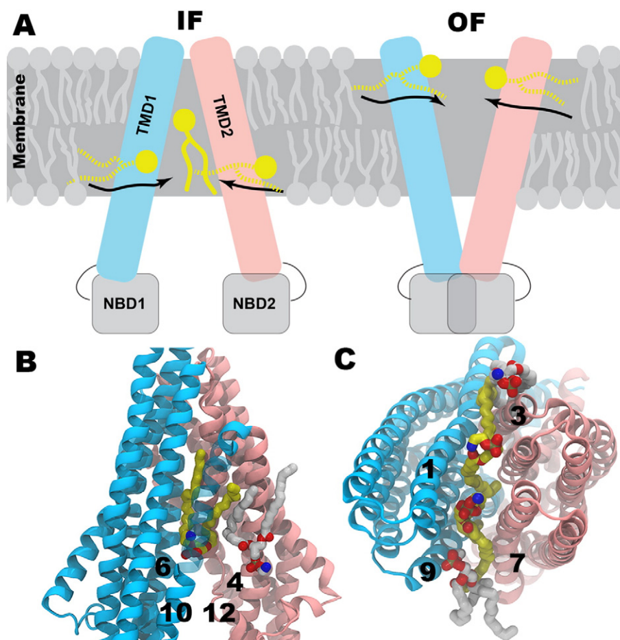
Fig. 8. Lipid binding to Pgp in its IF and OF states. A) Schematic representation of IF and OF conformations of Pgp. Half-inserted and fully inserted lipid molecules are shown in broken and solid yellow lines, respectively. B) Lipid binding through both probable drug entry portals (TM4&6 and TM10&12) in IF conformation. C) Lipid binding through both probable drug exit portals (TM1&3 and TM7&9) in OF conformation. TM helices are in cartoon representation while the initial and final conformations of lipid molecules are in white and yellow sticks, respectively. Hydrogen atoms are not shown for clarity.
