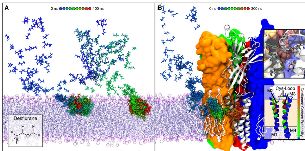
Fig. 5. Membrane partitioning of anesthetics facilitates binding to modulation sites of ion channels. A) Simulating high concentrations of desflurane (43 desflurane molecules, 1:5 ratio with lipid) demonstrated partitioning to the amphipathic glycerol region of the membrane within 100 ns. Two different paths of desflurane are shown, colored by simulation time, which exemplify membrane partitioning of inhaled anesthetics. B) Simulations employing high concentrations of desflurane were used to “flood” the GLIC protein embedded in a POPC membrane. Following the rapid partitioning of desflurane molecules into the membrane, several molecules spontaneously bound to the transmembrane domain, revealing an inner and outer binding site. The desflurane molecule forms several non-specific contacts within the inner binding site (top inset). Notably, the binding site near the same location within the membrane where desflurane partitions (bottom inset).
