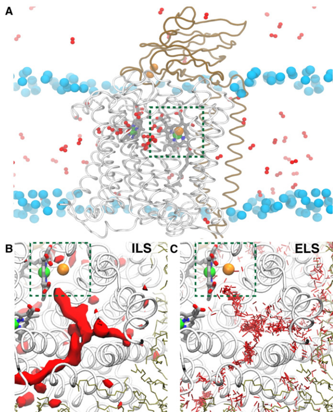
Fig. 3. Protein tunnels facilitate the rapid delivery of O_2 in CcO ba_3 . A) A side-view image of an O_2 simulation in CcO ba_3 illustrates the entry of substrate O_2 to CcO ba_3 from the membrane. Small red balls represent O_2 molecules distributed during the simulations. Dashed green box highlights the catalytic site of O_2 , consisting of a heme iron (green ball) and a copper ion (orange ball). Cyan spheres represent phosphorus atoms of membrane lipids. B) Top-view image highlight highly favorable O_2 binding regions calculated from ILS. The red surfaces correspond to the partitioning \Delta G isosurface of -3.0 kcal/mol. C) Top-view image highlights the collection of O_2 molecules that partition in the protein during ELS simulations.
