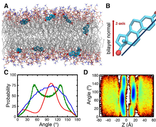
Fig. 6. Partitioning profile of estradiol in a POPC membrane. A) Snapshot after 200 ns illustrating multiple copies of estradiol in their preferred locations and orientations. The membrane consisted of POPC lipids and water molecules have been omitted for clarity. Estradiol is shown in stick (licorice) representation (C, cyan; O, red). B) To describe the orientation of the estradiol within the bilayer, an axis was defined pointing from O-17 to O-3, and an angle was measured with respect to the bilayer normal. C) The angle distribution of estradiol is shown in the lipid bilayer (red) or in bulk solution (blue). The angle distribution computed for an isotropic system (green) is shown for reference. D) Dependence of probability function for orientation of estradiol in the bilayer; the probability is shown in 2D plot, where the color changes from red to blue with increasing probability.
