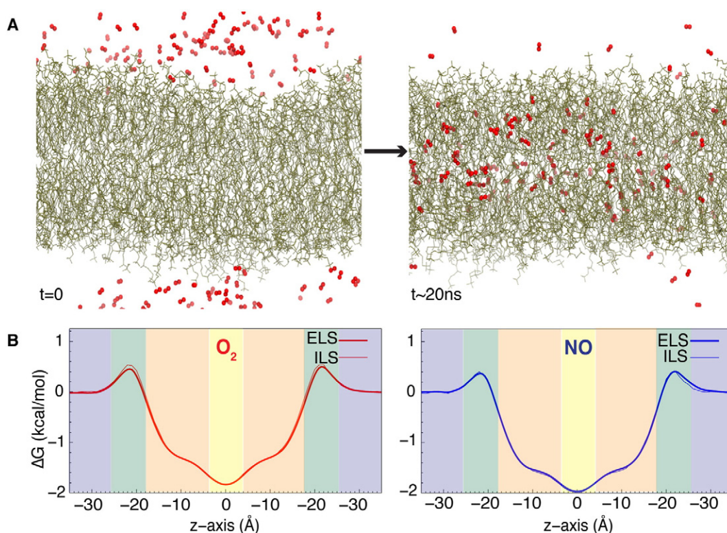
Fig. 2. Favorable membrane partitioning of gases. A) Illustration of the partitioning of gas molecules into the membrane from the aqueous solution from an ELS trajectory. This illustration is taken from a flooding simulation of O_2 molecules (shown in red) which are initially distributed in the aqueous solution. As time progresses, O_2 molecules spontaneously enter the membrane and become steadily distributed in both aqueous and lipid phases. More O_2 molecules localize in the membrane than in the aqueous solution. B) Partitioning free energy profiles of O_2 and NO gases in a POPC bilayer calculated using ELS trajectories and ILS. Shaded blue boxes in each plot represent the aqueous solution. Shaded green boxes represent the polar head group of the membrane. Shaded orange boxes represent hydrophobic lipid tails region. A shaded yellow box represents the interface between two membrane leaflets.
