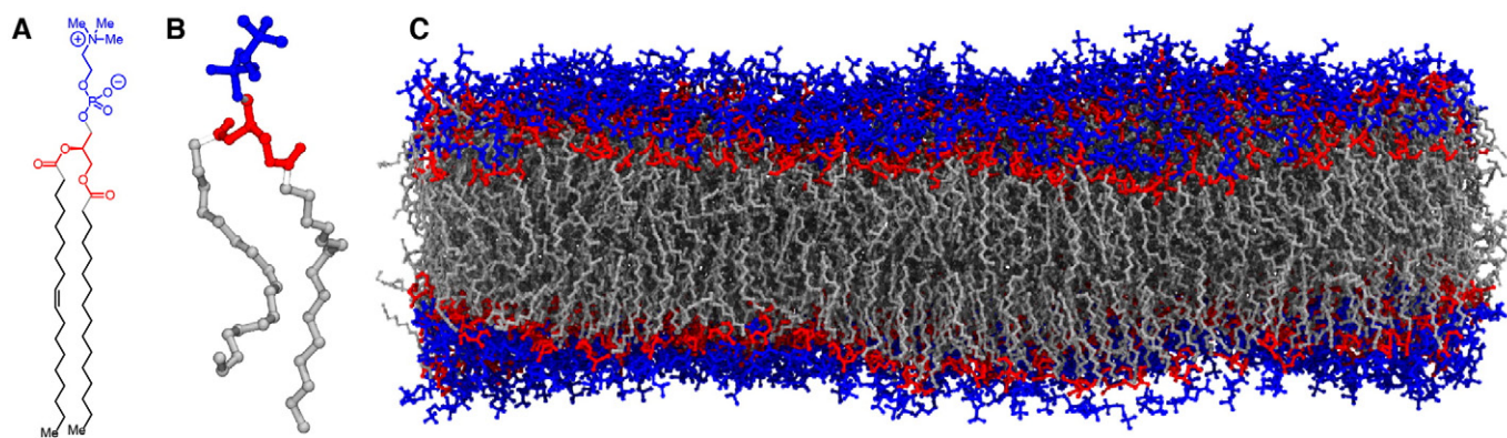
Fig. 1. Membrane structure is defined by the chemical structure of lipids. A) The chemical structure of 1-palmitoyl-2-oleoyl- sn -glycero-3-phosphocholine (POPC), a prototypical lipid present in eukaryotic membranes, is comprised of a zwitterionic head group (blue), a polar glycerol group (red), and non-polar carbon tails (black/gray). B) A three-dimensional structure of an isolated phospholipid highlights the flexibility of the carbon tails which engenders the fluid and highly dynamic nature of membranes. C) By color coding the different chemical groups within each lipid, three distinct regions within a fully equilibrated POPC membrane become clear. The chemical details defined by small molecule interactions with the different lipid functional groups are major determinants of how molecules partition into the membrane.
