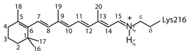
FIGURE 1 Schematic representation of all- trans retinal bound via a protonated Schiff base to Lys-216 in bR and its conventional atom numbering.
