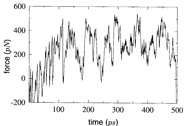
FIGURE 10 The time dependence of the applied force for a stiff cantilever f = 280 pN/ \text{\AA} , v = 0.015 \text{ \AA/ps} , and \gamma = 2000 ps pN/ \text{\AA} .
