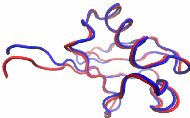
Figure 12: Initial and final states of ubiquitin after spatial alignment.
