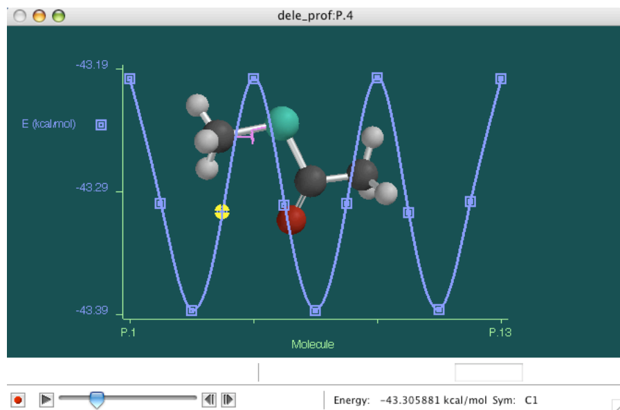
Figure 13: Dihedral energy profile results.
